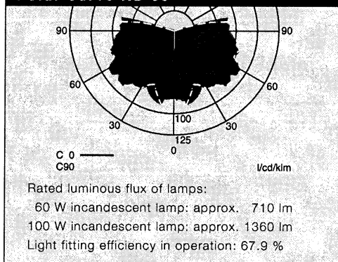
Polar curve AB 50
