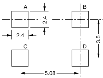
Figure 2) ECX-19A Land Pattern
