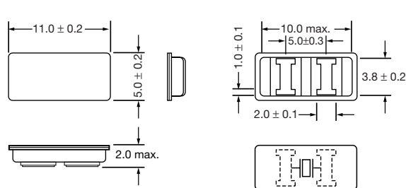
Figure 1) ECX-19A - Top, Side, Bottom and End views
