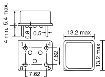
Figure 1) ECS-2200X Series – Side, Bottom and Top views
