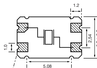
Figure 3) CSM-8B – Pad Configuration Bottom view
