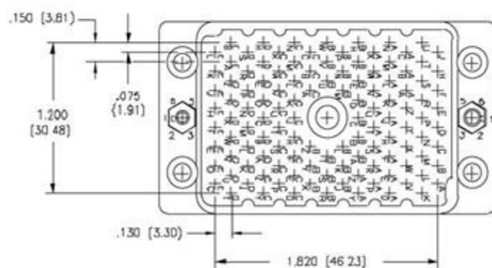
120 PIN PLUG
