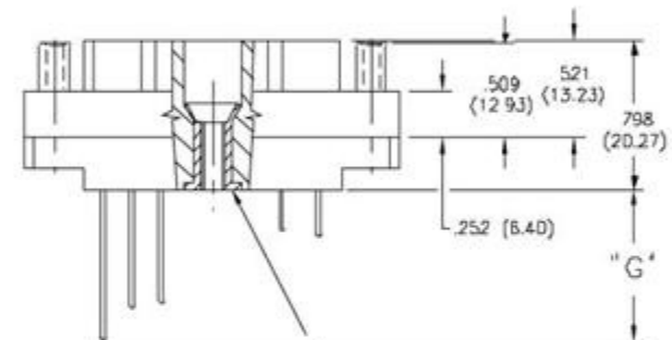
TYPICAL RECEPTACLE WITH LOCKNUT AND POLARIZING SOCKETS
