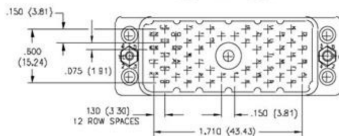
56 PIN PLUG
