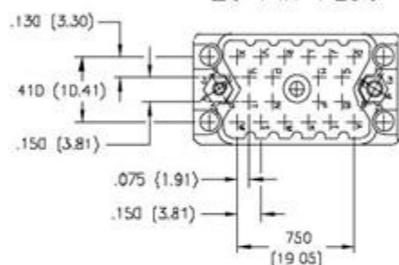
20 PIN PLUG
