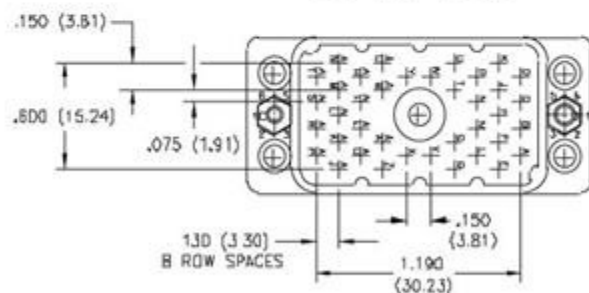
38 PIN PLUG
