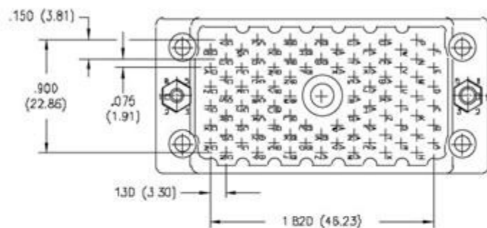
90 PIN PLUG
