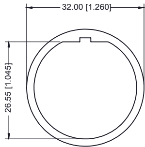
O-RING
