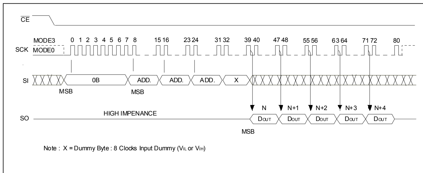
Figure 3 : HIGH-SPEED-READ SEQUENCE
