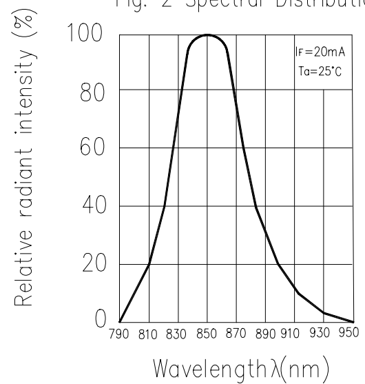
Fig. 2 Spectral Distribution
