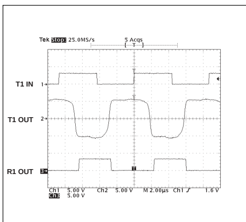
Figure 13. Loopback Test Circuit result at 235Kbps (All Drivers Fully Loaded)
