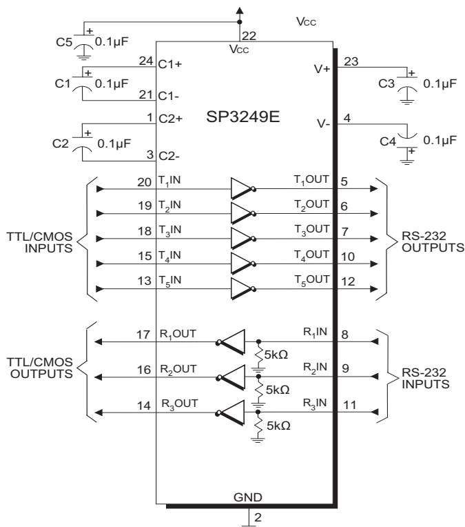
Figure 5. SP3249E Typical Operating Circuit
