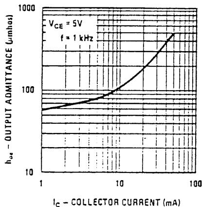
Output Admittance
