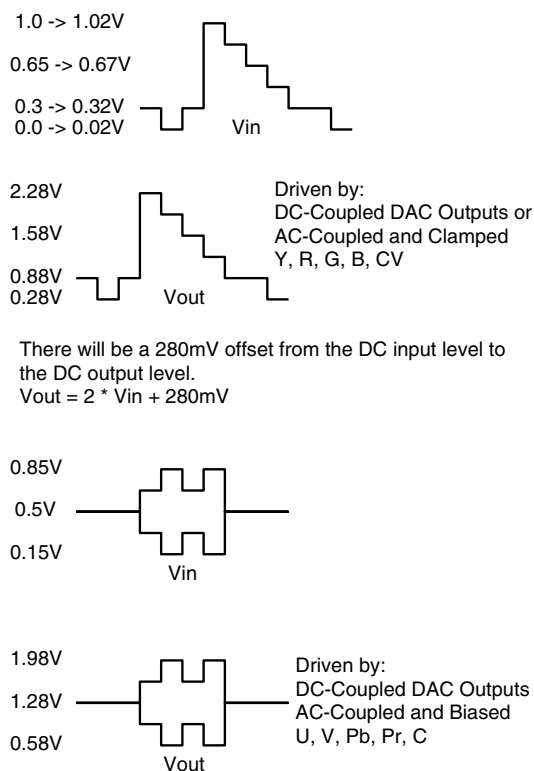
Figure 1. Typical Voltage Levels
