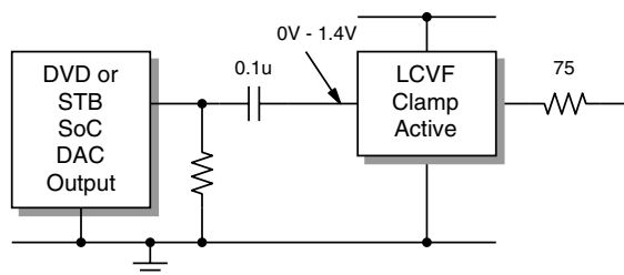
Figure 4. AC-coupled Inputs, DC-coupled Outputs
