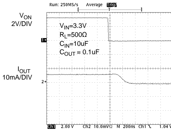
Figure 21. T OFF Response
