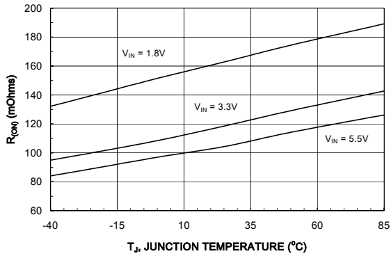
Figure 13. R_{(ON)} vs. Temperature
