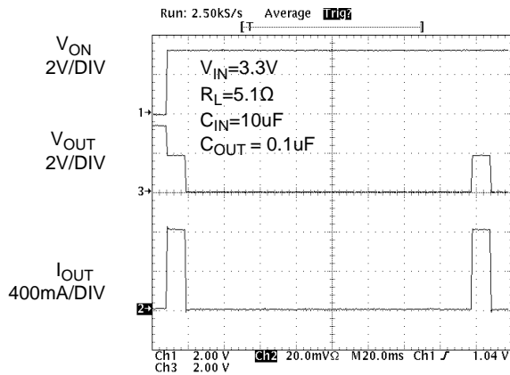
Figure 19. T RESTART Response
