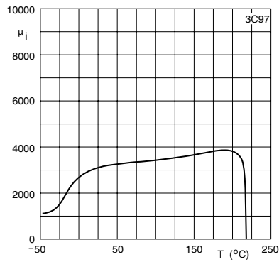
Fig. 2 Initial permeability as a function of temperature
