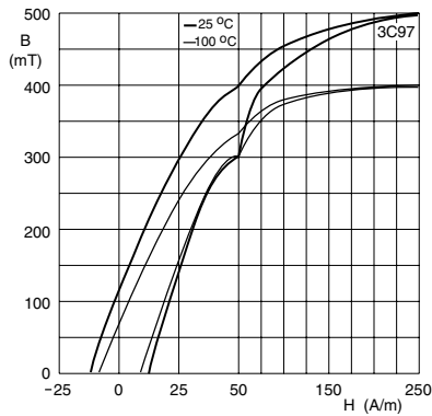
Fig. 3 Typical B-H loops
