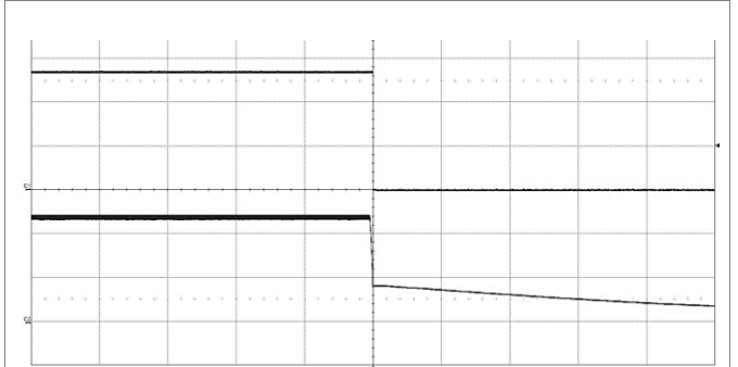
Shut-down enabled by disconnecting V_I at: T_{P1} = +25^\circ\text{C} , V_I = 48\text{ V} , I_O = 0.463\text{ A} resistive load. Top trace: output voltage (20 V/div.). Bottom trace: input voltage (20 V/div.). Time scale: (200 ms/div.).
