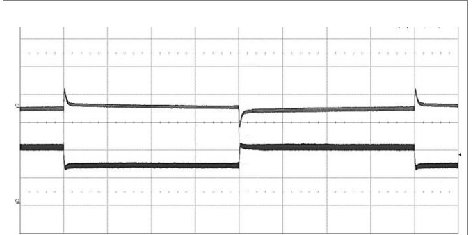
Output voltage response to load current step-change (0.231-0.347-0.231 A) at: T_{P1} = +25^\circ\text{C} , V_I = 48\text{ V} . Top trace: output voltage (500 mV/div.). Bottom trace: load current (200 mA/div.). Time scale: (2 ms/div.).
