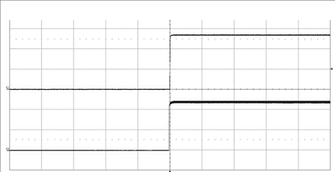
Start-up enabled by connecting V_I at: T_{P1} = +25^\circ\text{C} , V_I = 48\text{ V} , I_O = 0.463\text{ A} resistive load. Top trace: output voltage (20 V/div.). Bottom trace: input voltage (20 V/div.). Time scale: (200 ms/div.).
