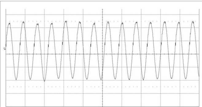
Output voltage ripple at: T_{P1} = +25^{\circ}\text{C} , V_I = 48\text{ V} , I_O = 0.625\text{ A} resistive load. Trace: output voltage (20 mV/div.). Time scale: (5 µs/div.). 20MHz bandwidth
