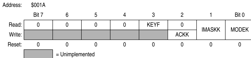
Figure 18-3. Keyboard Status and Control Register (KBSCR)
