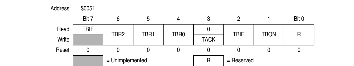
Figure 10-2. Timebase Control Register (TBCR)
