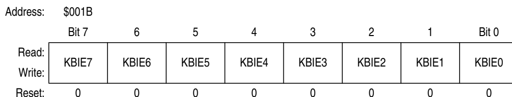
Figure 18-4. Keyboard Interrupt Enable Register (KBIER)
