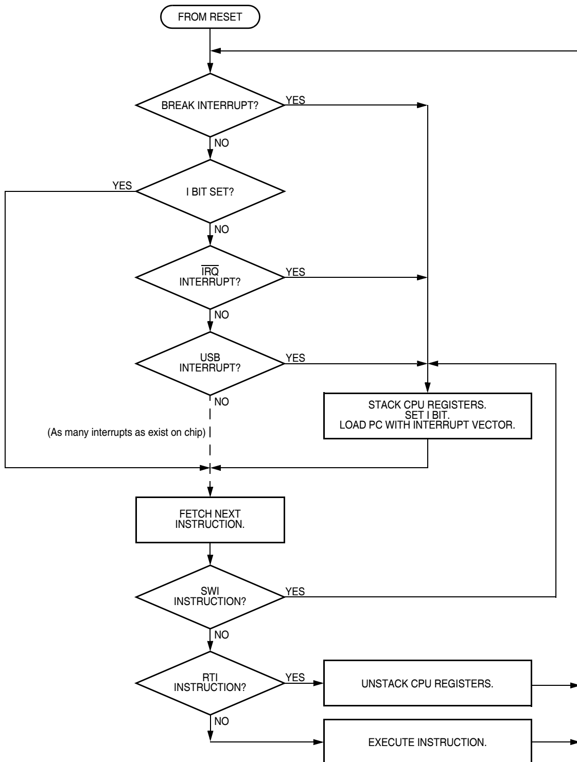
Figure 7-9. Interrupt Processing
