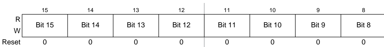
Figure 7-19. Timer Input Capture/Output Compare Register 0 High (TC0)
