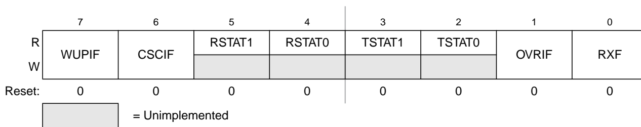
Figure 10-8. MSCAN Receiver Flag Register (CANRFLG)
