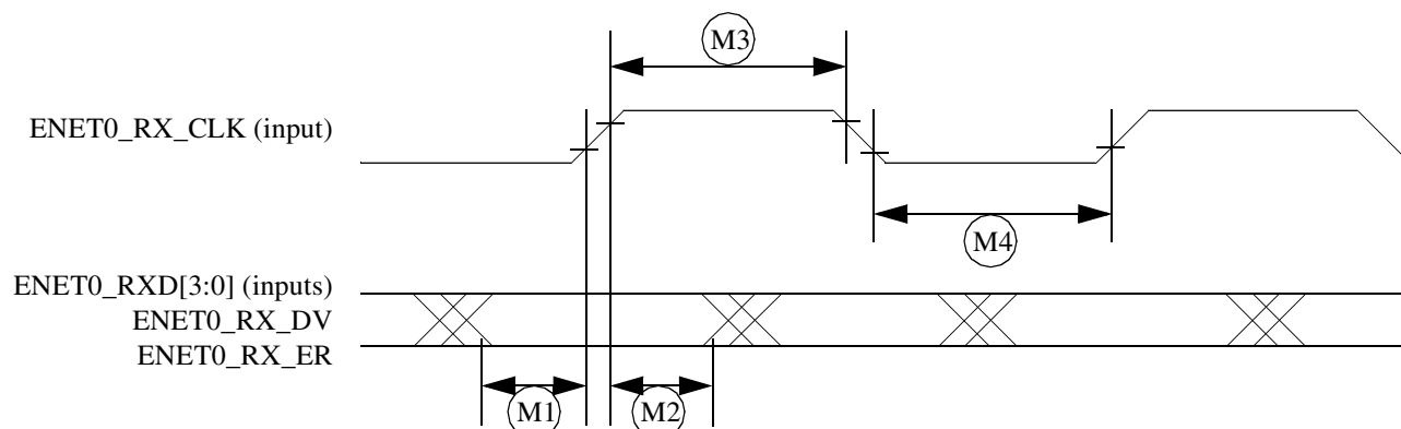
Figure 9. MII Receive Signal Timing Diagram
