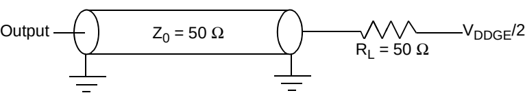
Figure 29. AC Test Load
