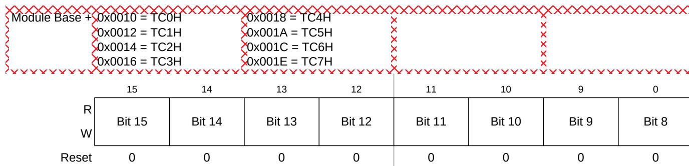
Figure 14-22. Timer Input Capture/Output Compare Register x High (TCxH)
