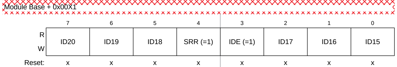
Figure 8-27. Identifier Register 1 (IDR1) — Extended Identifier Mapping
