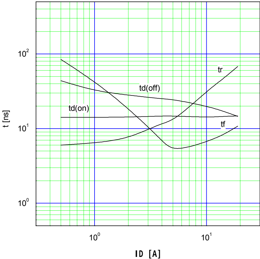
Typical Switching Characteristics vs. I_D t=f(I_D): V_{cc}=300\text{V}, V_{GS}=10\text{V}, R_G=10\text{ }\Omega
