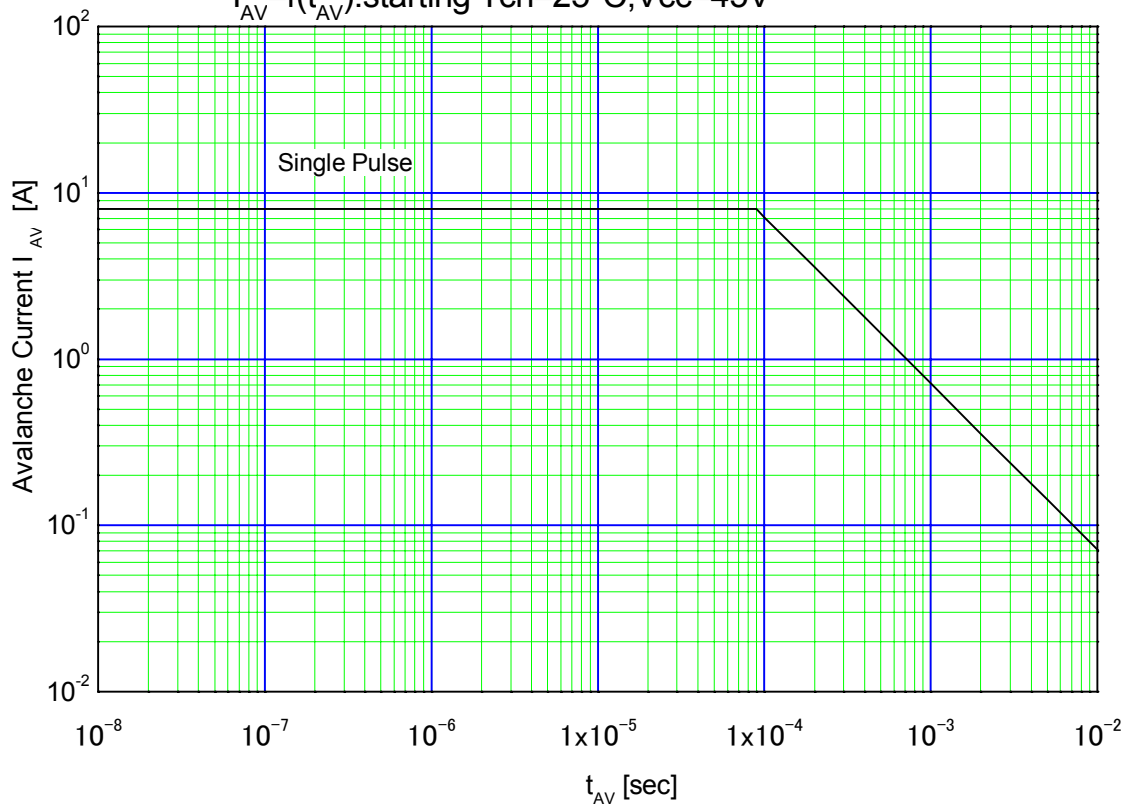
Maximum Avalanche Current Pulsewidth I_{AV}=f(t_{AV}): \text{starting Tch}=25^{\circ}C, V_{CC}=45V
