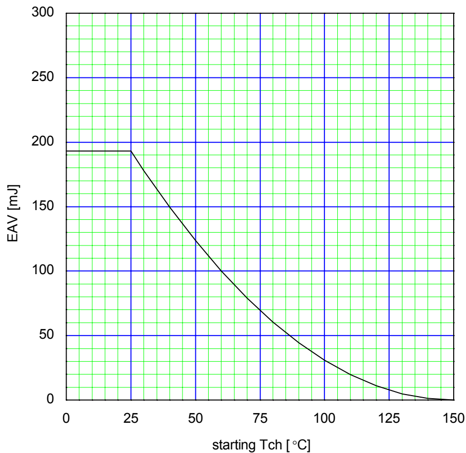
Maximum Avalanche Energy vs. starting Tch E(AV)=f(\text{starting Tch}):V_{CC}=45V, I(AV)\leq 8A
