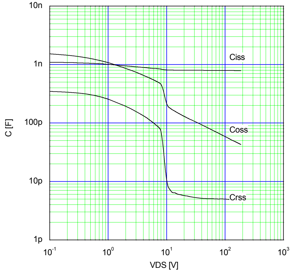
Typical Capacitance C=f(V_{DS}): V_{GS}=0V, f=1\text{MHz}
