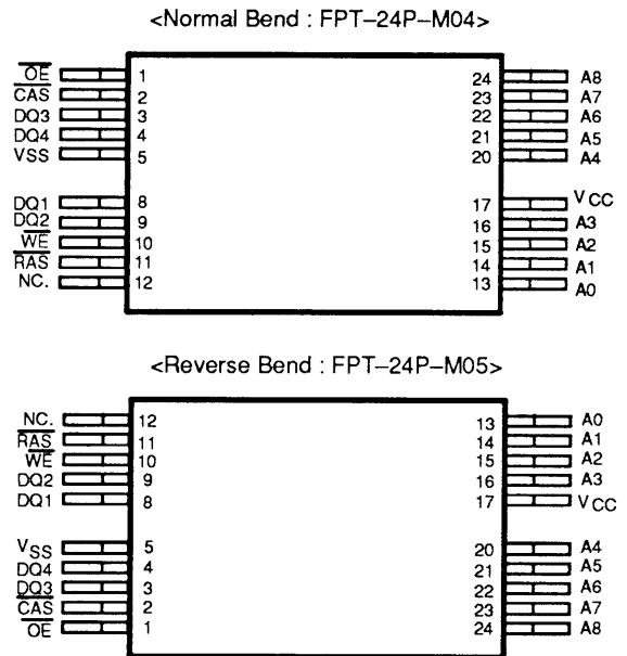
24-Pin FPT : (TOP VIEW)
