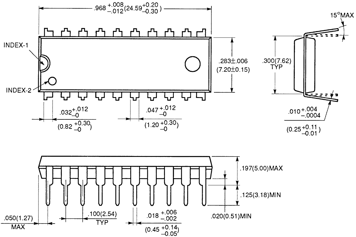
20-Lead Plastic Dual In-Line Package (Case No.: DIP208P-M03)
