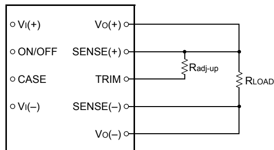
Figure 37. Circuit Configuration to Increase Output Voltage.
