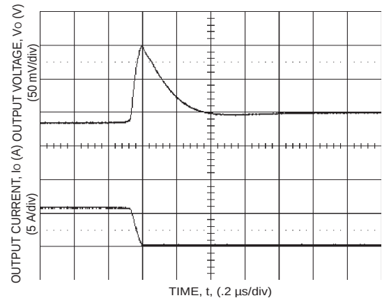
Figure 4. Transient Response to Step decrease in Load from 50% to 25% of Full Load ( V_I = 48 Vdc).
