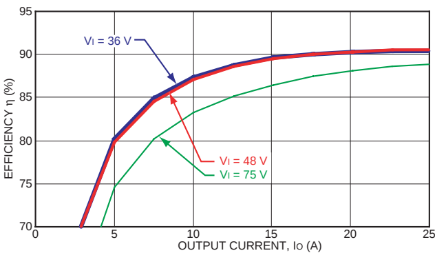
Figure 20. Converter Efficiency vs. Output Current.
