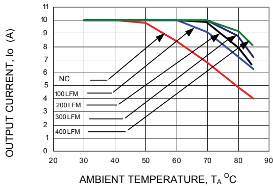
Figure 19. Derating Output Current versus Local Ambient Temperature and Airflow ( V_{in} = 12.0\text{ Vdc} , V_o = 0.75\text{ Vdc} ).
