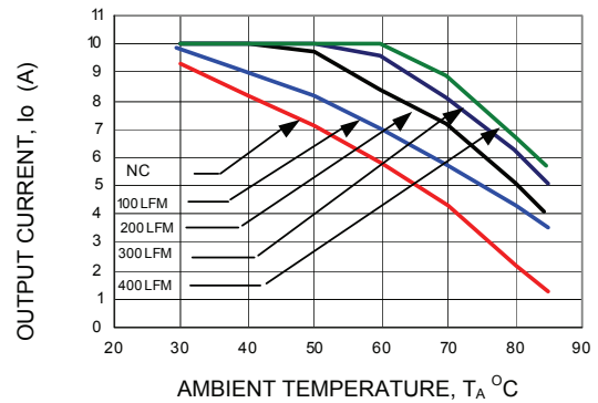
Figure 22. Derating Output Current versus Local Ambient Temperature and Airflow ( V_{in} = 12.0\text{ Vdc} , V_o = 5.0\text{ Vdc} ).
