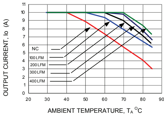
Figure 20. Derating Output Current versus Local Ambient Temperature and Airflow ( V_{in} = 12.0\text{ Vdc} , V_o = 1.8\text{ Vdc} ).
