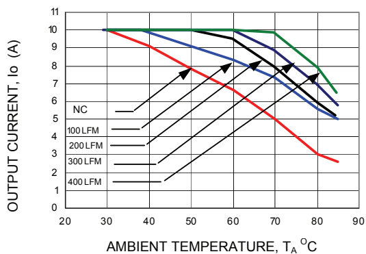
Figure 21. Derating Output Current versus Local Ambient Temperature and Airflow ( V_{in} = 12.0\text{ Vdc} , V_o = 3.3\text{ Vdc} ).
