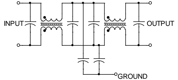
Figure 4. Internal Schematic
