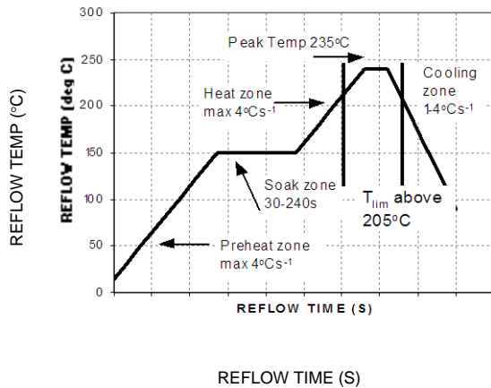
Figure 13. Reflow Profile for Tin/Lead (Sn/Pb) process.
