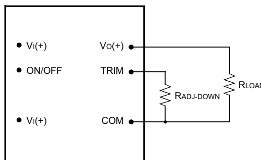
Figure 23. Circuit Configuration to Decrease Output Voltage
