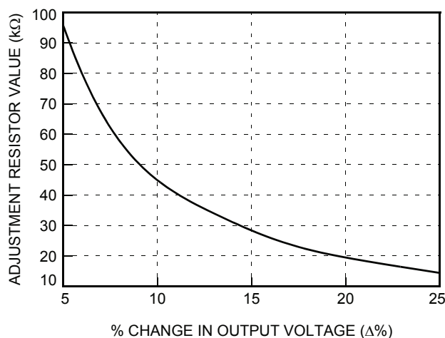
Figure 24. Resistor Selection for Decreased Output Voltage for V O1
