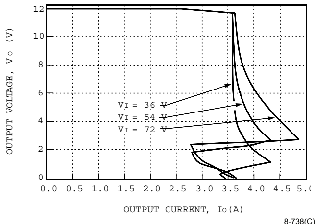
Figure 7. JW030B-M Typical Output Characteristics
