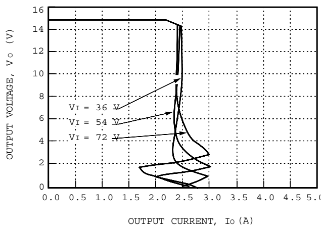
Figure 8. JW030C-M Typical Output Characteristics
