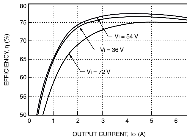
Figure 11. JW030F-M Typical Converter Efficiency vs. Output Current
