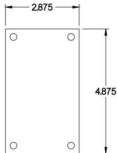
INNER PANEL
