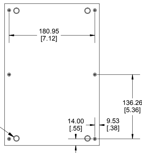
BOTTOM VIEW OF ENCLOSURE
