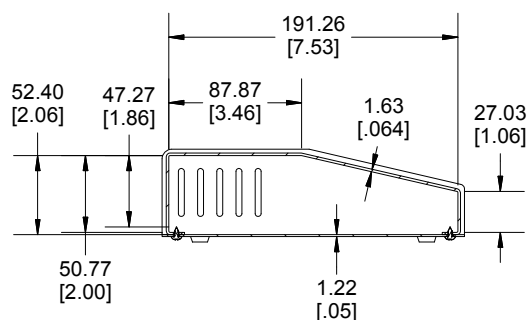
SECTION B-B END VIEW
