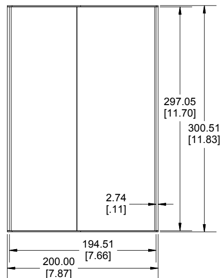
END VIEW OF ENCLOSURE
