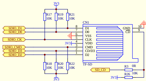
SD Card
