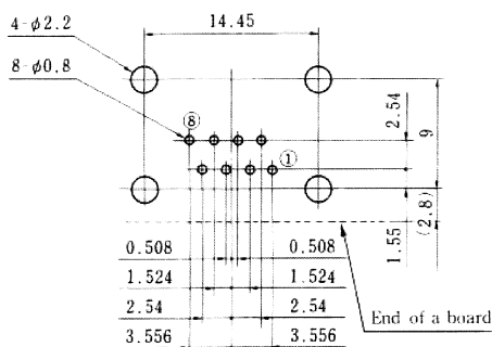
Board mounting dimensional drawing (connector side)
