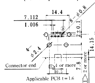
Reference mounting dimensions (PCB component side)
