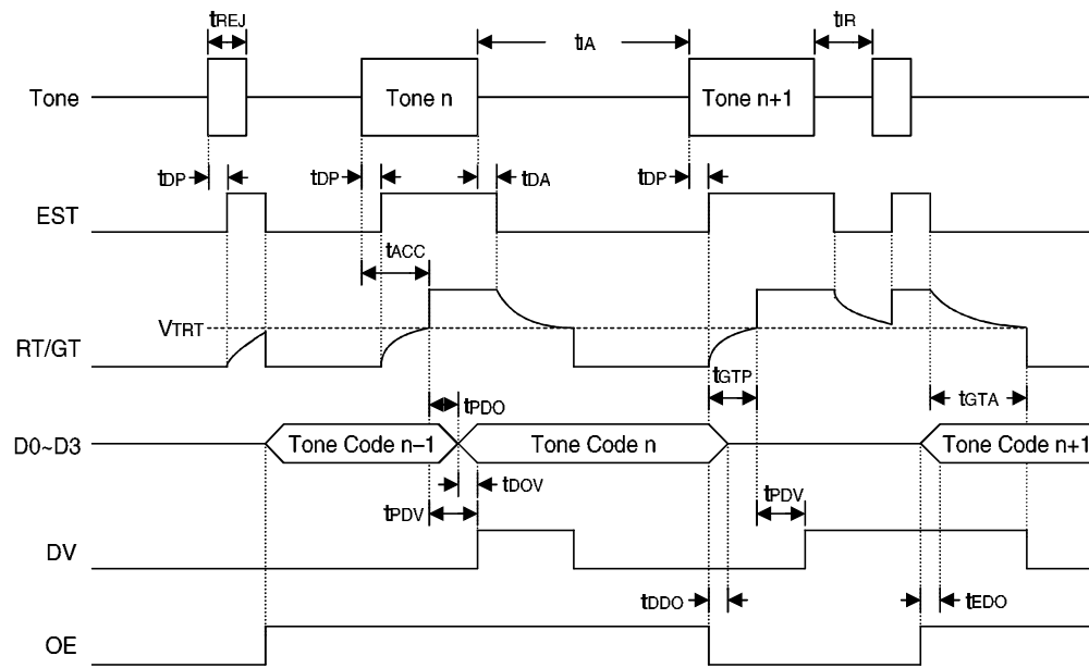
Figure 3. Steering timing
