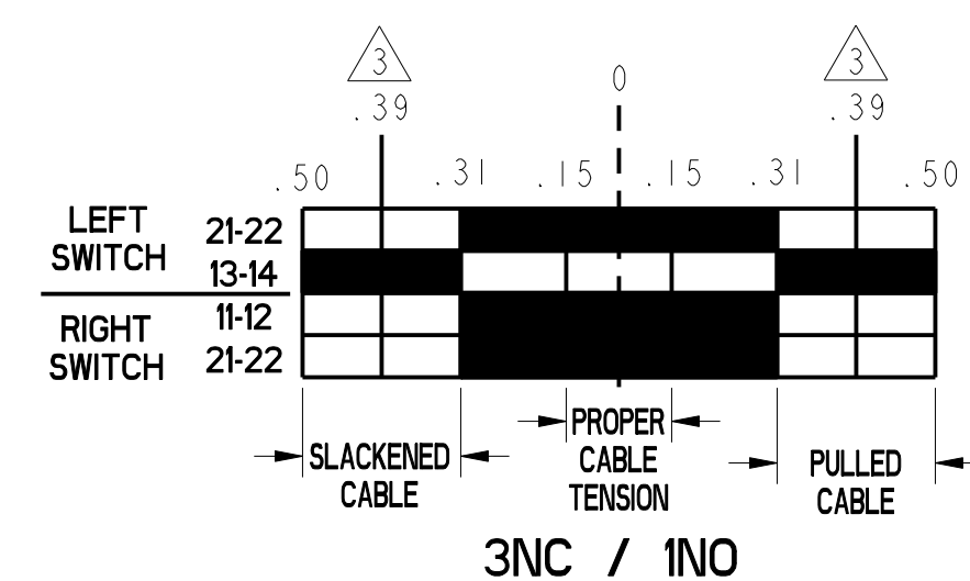
SHAFT TRAVEL CHART
