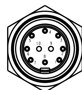
10 PIN BRAD-HARRISON CONNECTOR DETAIL
