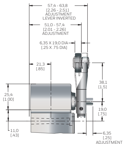
Figure 13. LS2Z51 Type Levers Cam Tracking
