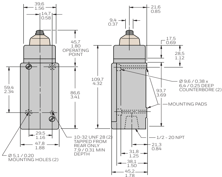
Figure 18. LS2 Series Top Pin Plunger (mm [in])
