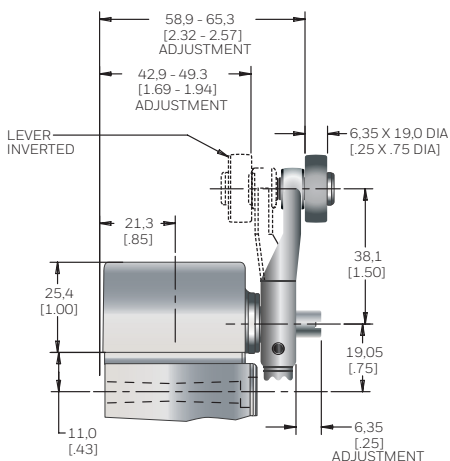
Figure 15. LS2Z54 Type Levers Cam Tracking
