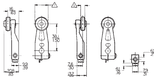
Front mounting
