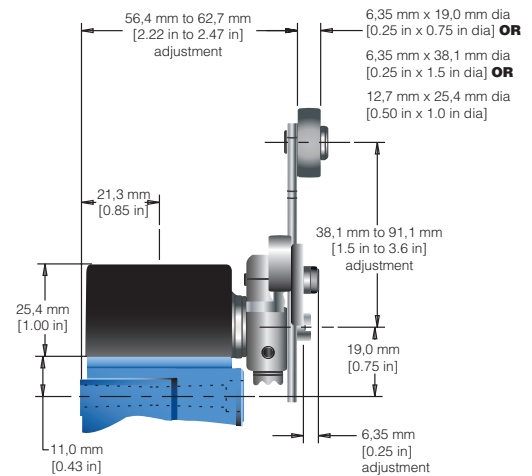
Figure 7. LSZ52 type levers cam tracking
