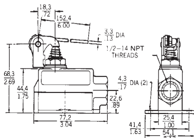
Flange mount without boot seal
