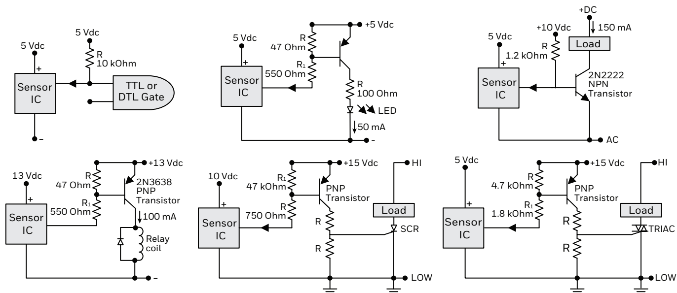
Figure 3. Circuit Diagrams
