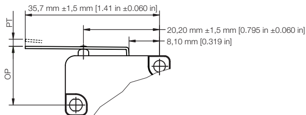
Figure 20. V15 Series A02/Standard Straight Lever
