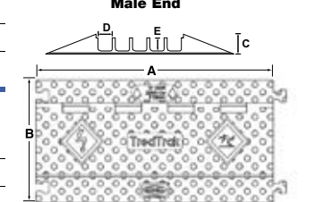
Male End
