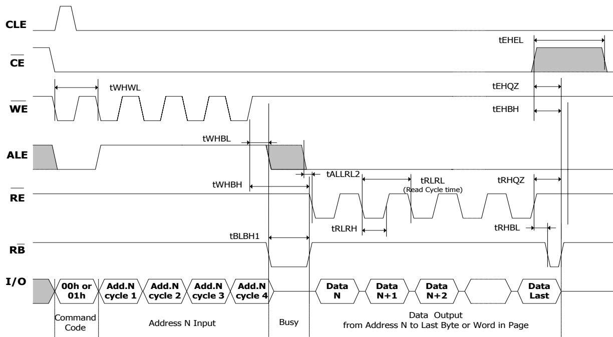
Figure 27. Read A/ Read B Operation AC Waveform
