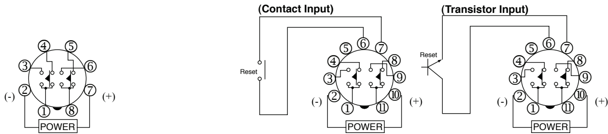
Delayed DPDT Output
