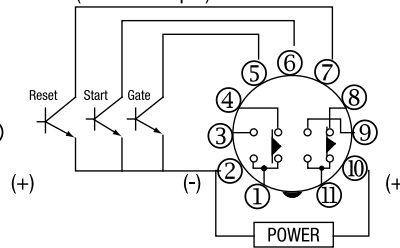
(Transistor Input)
