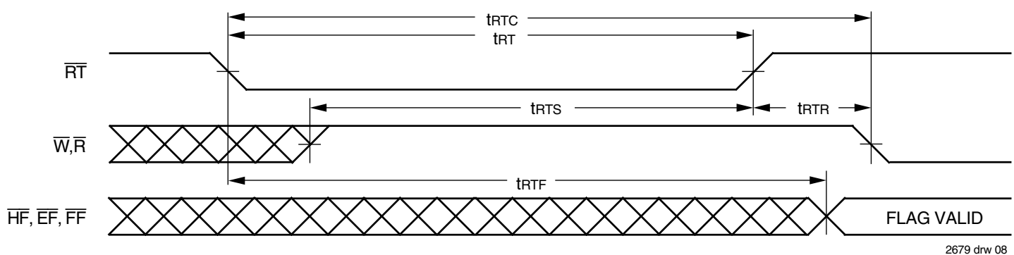
Figure 6. Retransmit
