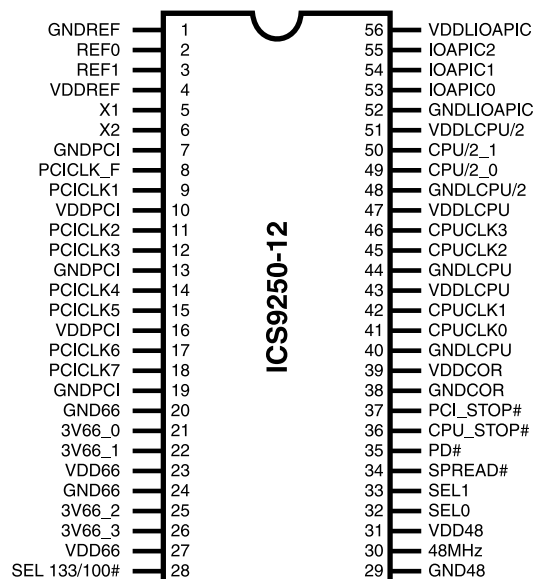
56-pin SSOP
