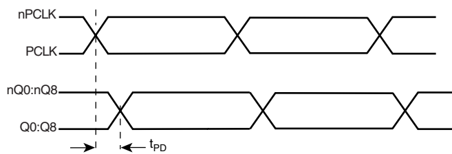
PROPAGATION DELAY
