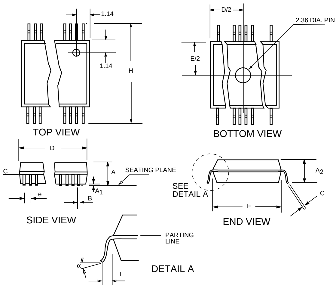
SSOP Package
