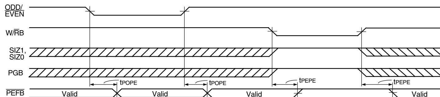
Figure 17. ODD/ \overline{EVEN} , \overline{W/RB} , SIZ1, SIZ0, and PGB to \overline{PEFB} Timing
