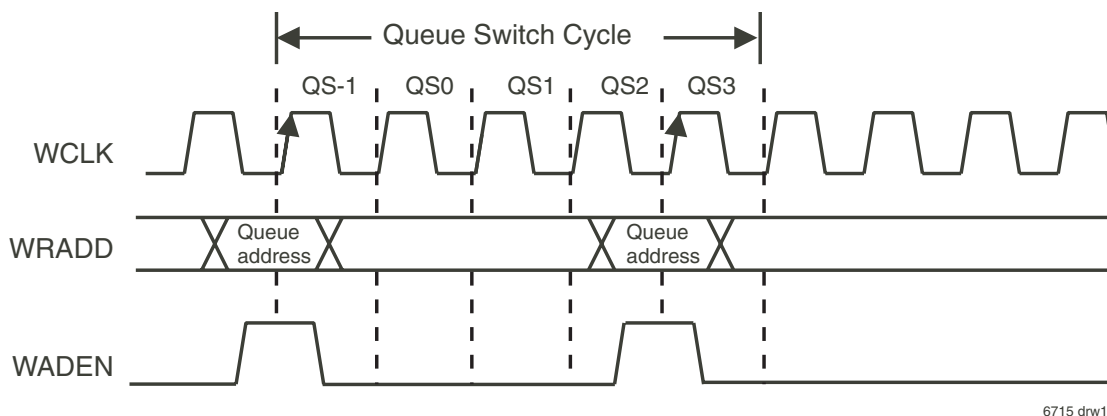
Figure 7. Write Port Switching Queues Signal Sequence
